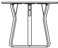
Theo table round diameter 750 height 740
