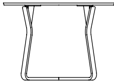
Theo table square width/depth 750 x 750 width/depth 900 x 900 height 740
