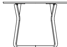
Theo table round diameter 900/1050/1200 height 740
