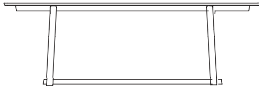
Theo table rectangle width/depth 1400 x 750 width/depth 1800 x 750 width/depth 1800 x 900 height 740
